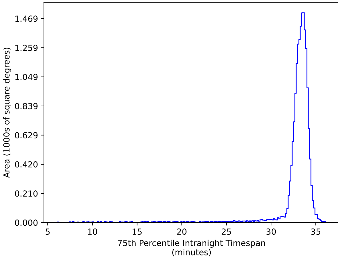
baseline_v3.3_10yrs WFD ug bands: 75th Percentile Intranight Timespan
