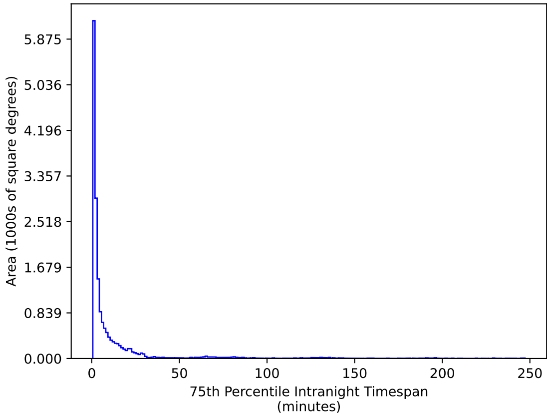
baseline_v3.3_10yrs WFD u band: 75th Percentile Intranight Timespan
