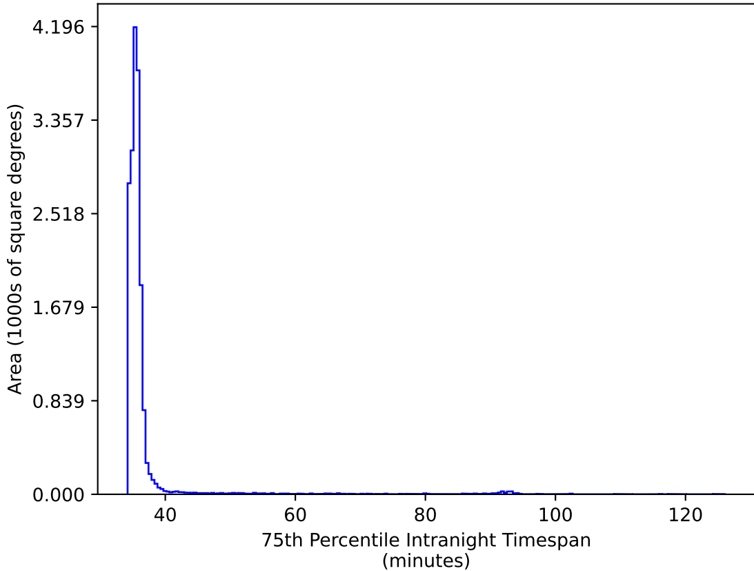
baseline_v3.3_10yrs WFD ri bands: 75th Percentile Intranight Timespan
