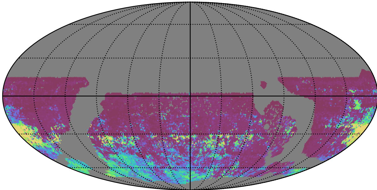
baseline_v3.3_10yrs WFD r band: 75th Percentile Intranight Timespan
