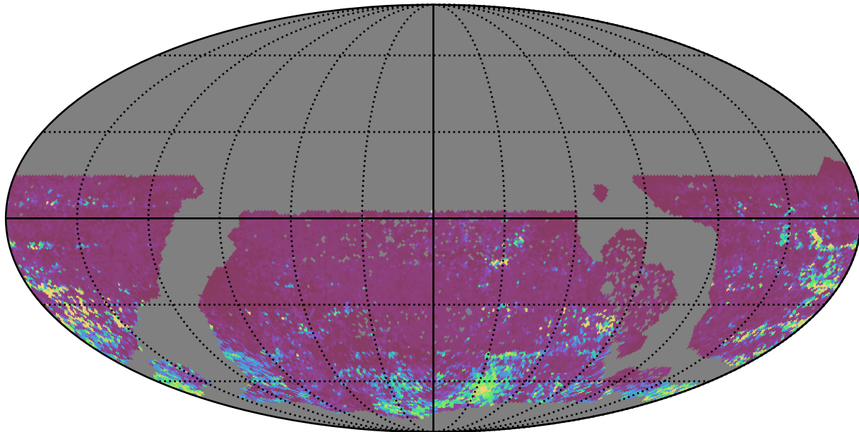
baseline_v3.3_10yrs WFD i band: 75th Percentile Intranight Timespan
