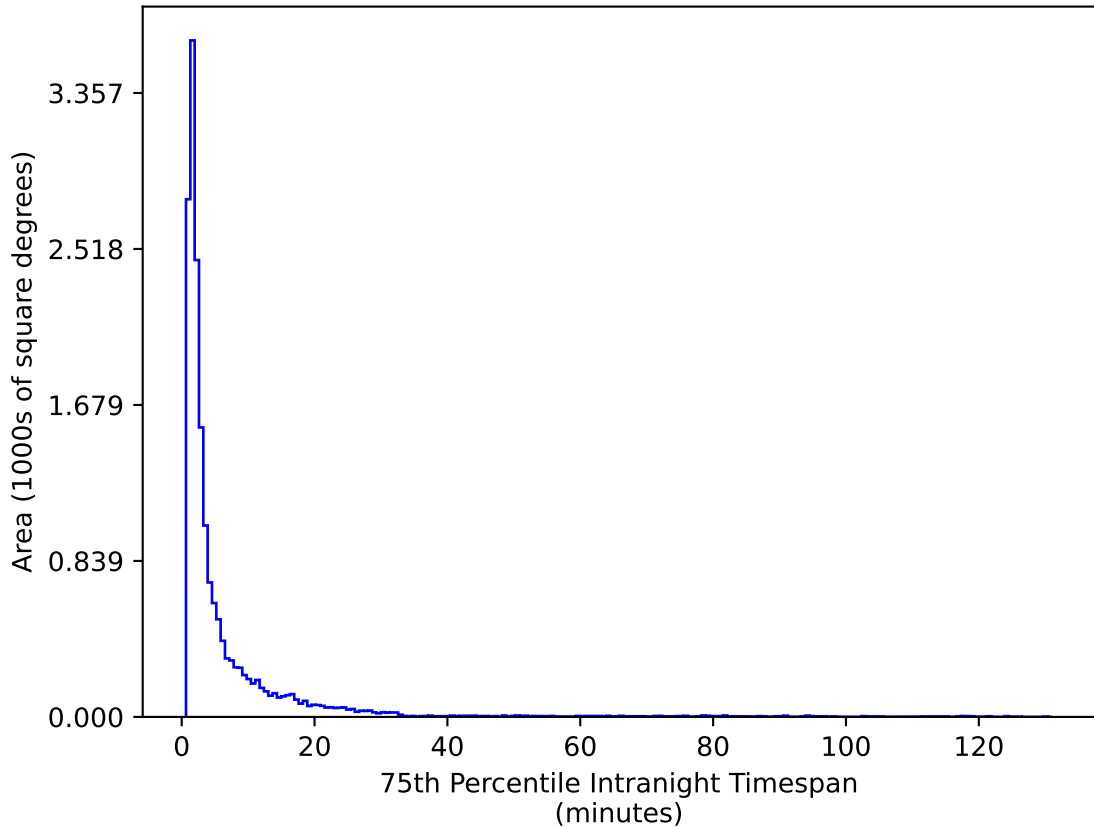
baseline_v3.3_10yrs WFD g band: 75th Percentile Intranight Timespan
