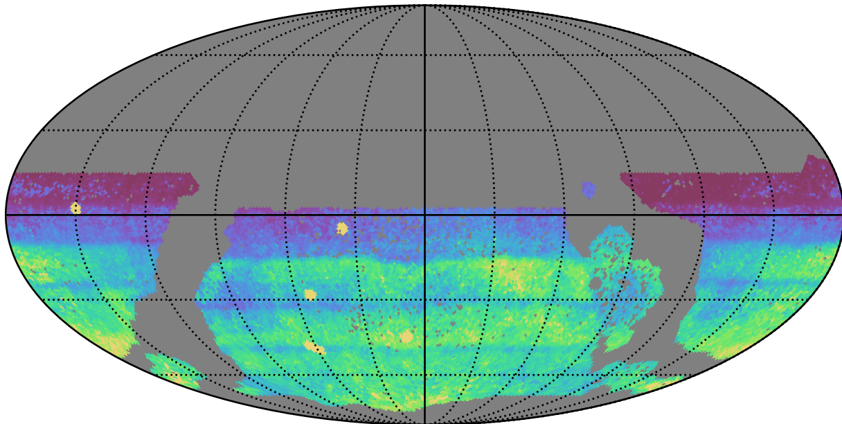
baseline_v3.3_10yrs WFD all bands: 75th Percentile Intranight Timespan
