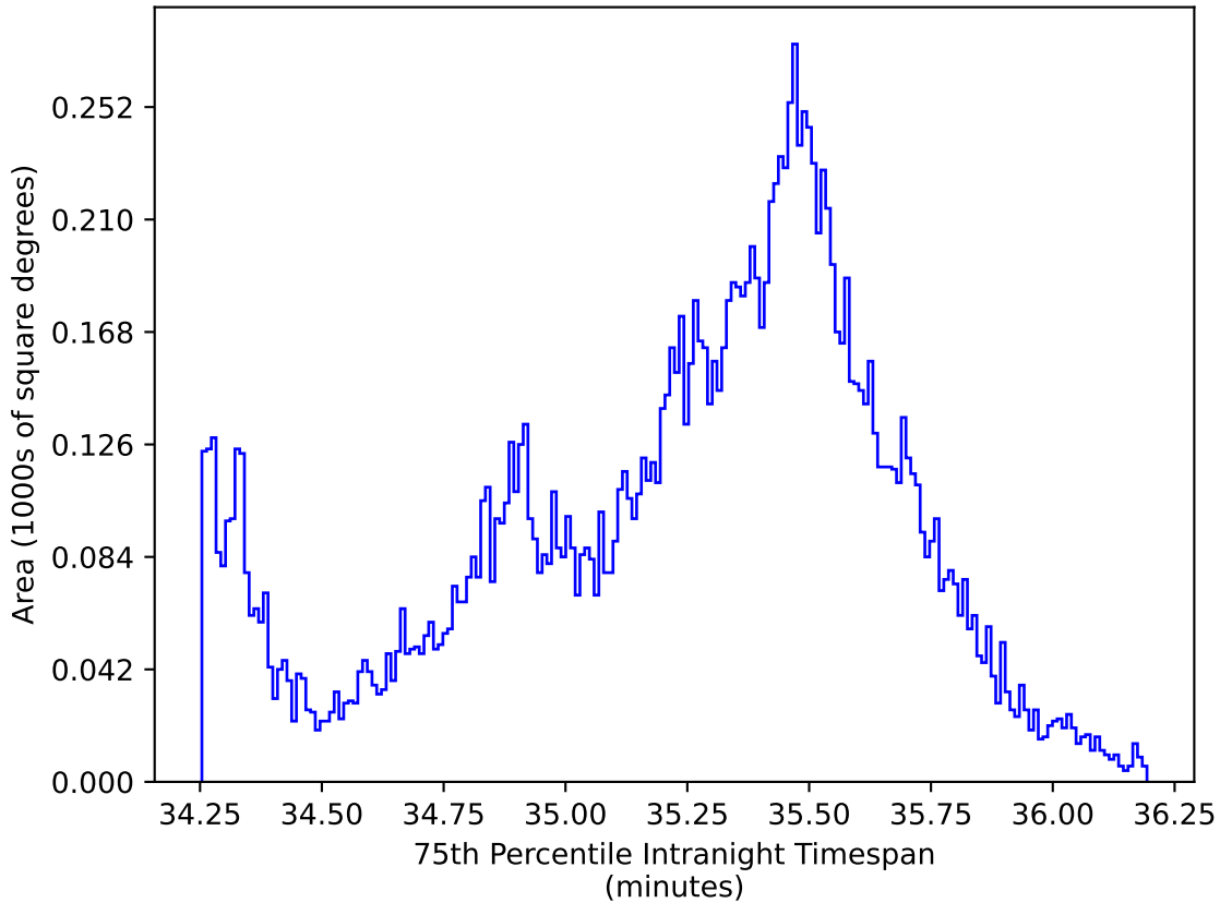
baseline_v3.3_10yrs WFD all bands: 75th Percentile Intranight Timespan
