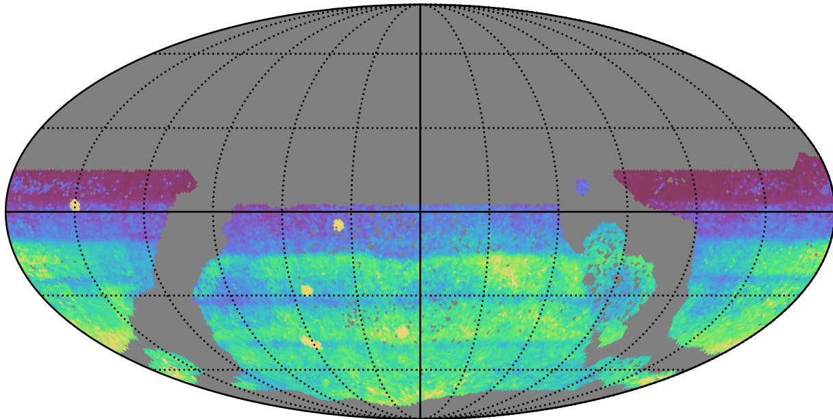
baseline_v3.3_10yrs WFD: 75th Percentile Intranight Timespan
