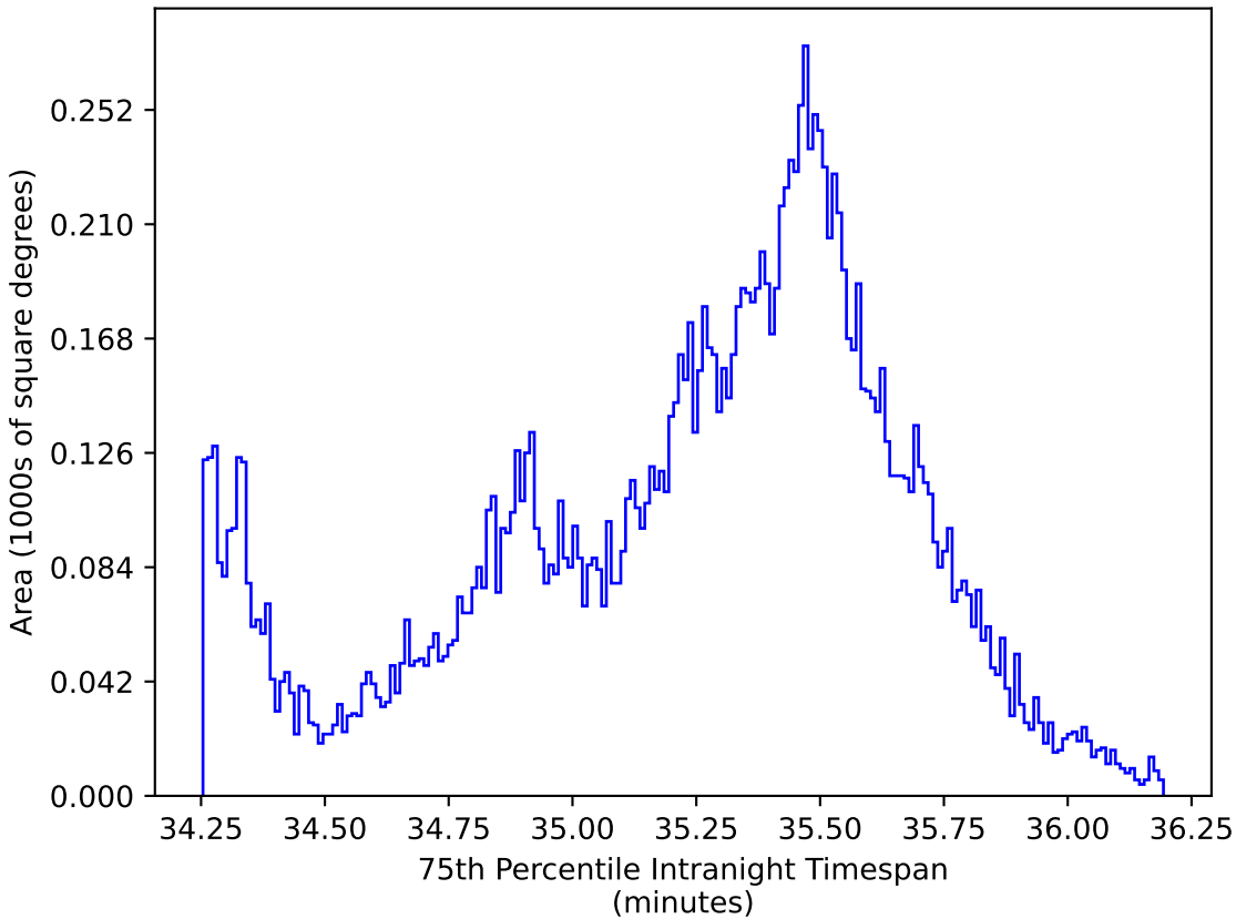
baseline_v3.3_10yrs WFD: 75th Percentile Intranight Timespan
