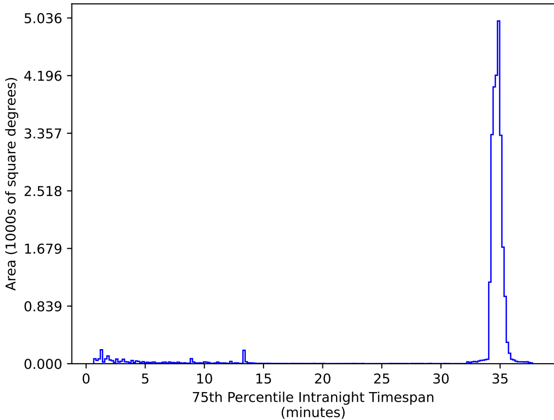
baseline_v3.3_10yrs All sky zy bands: 75th Percentile Intranight Timespan
