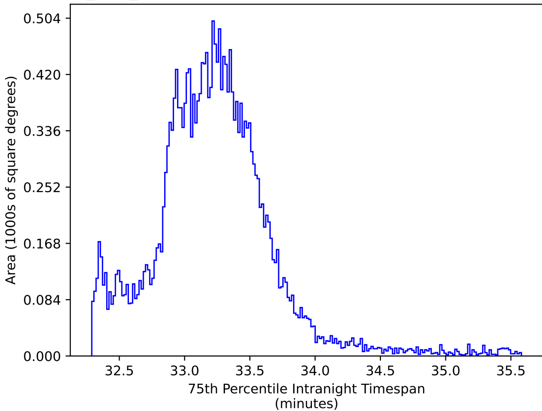
baseline_v3.3_10yrs All sky y band: 75th Percentile Intranight Timespan
