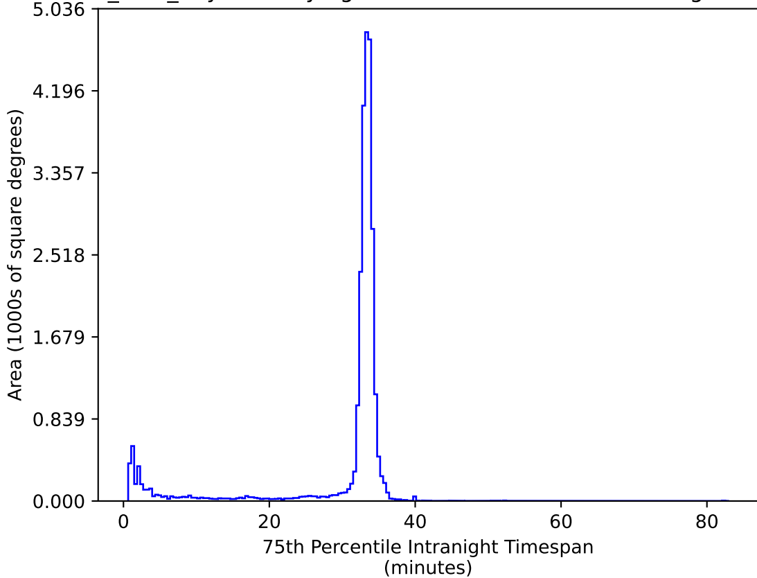
baseline_v3.3_10yrs All sky ug bands: 75th Percentile Intranight Timespan
