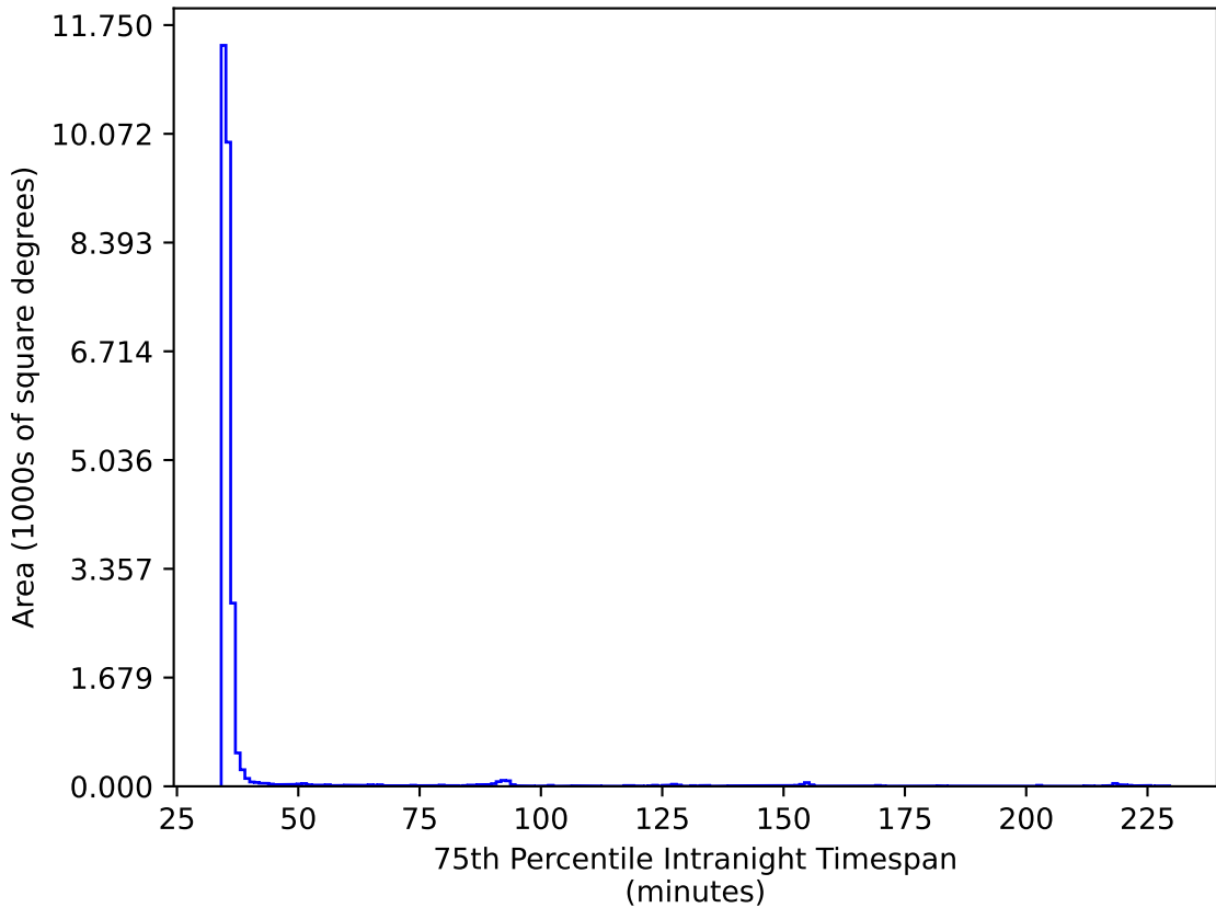
baseline_v3.3_10yrs All sky ri bands: 75th Percentile Intranight Timespan
