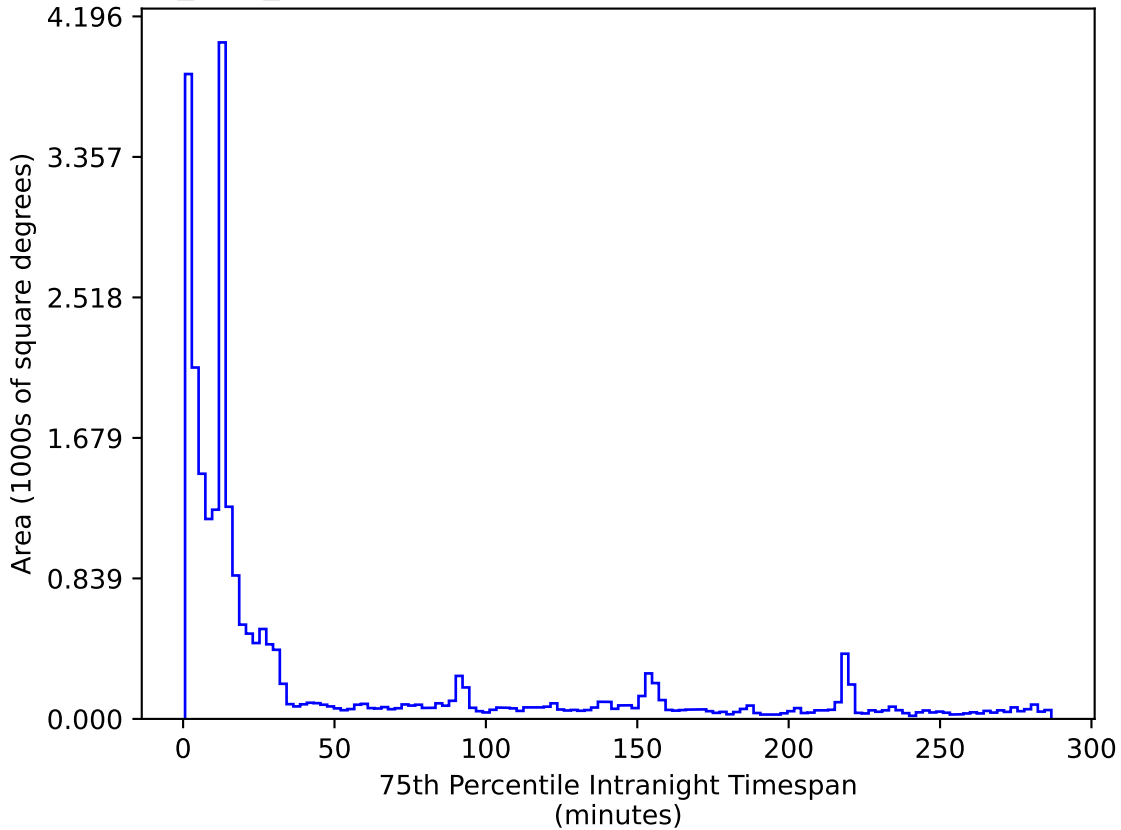
baseline_v3.3_10yrs All sky r band: 75th Percentile Intranight Timespan
