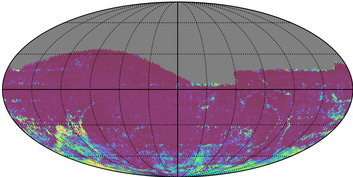
baseline_v3.3_10yrs All sky i band: 75th Percentile Intranight Timespan
