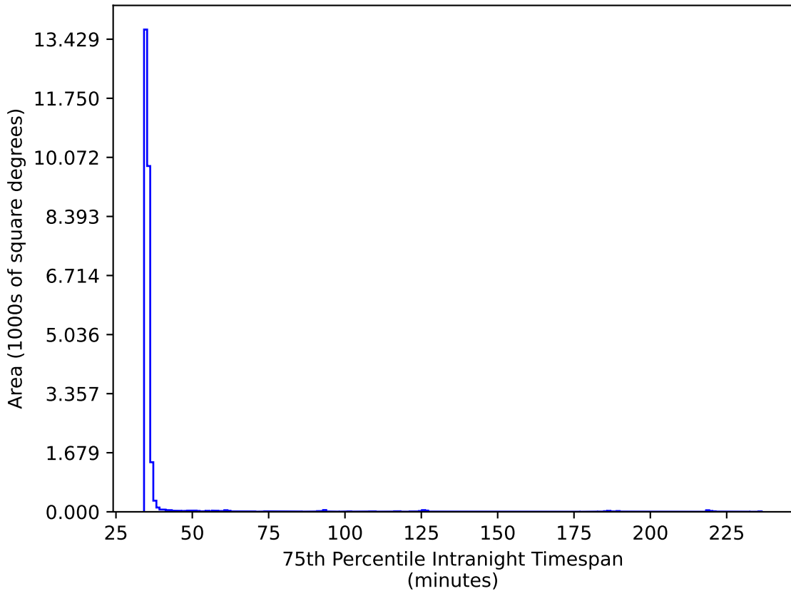
baseline_v3.3_10yrs All sky gr bands: 75th Percentile Intranight Timespan
