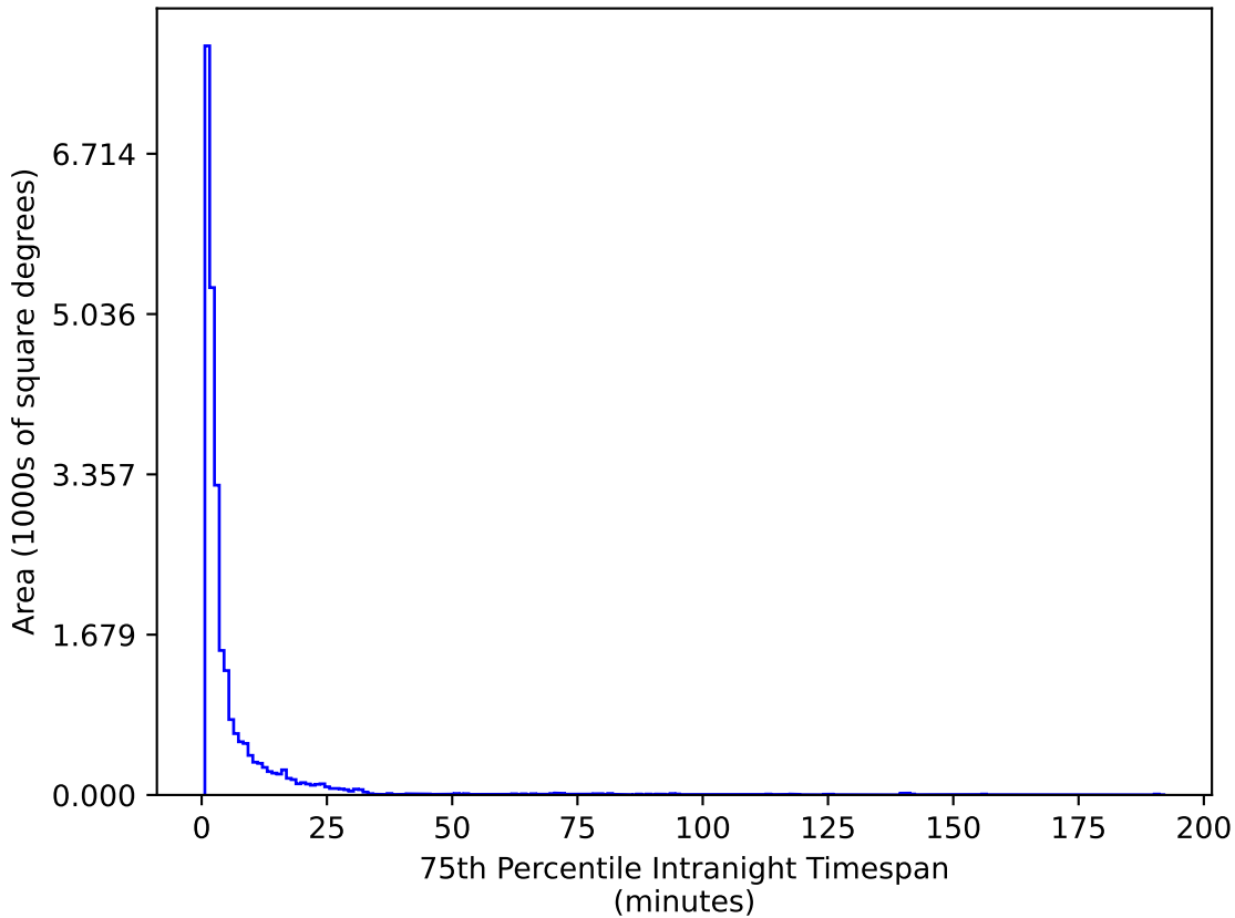
baseline_v3.3_10yrs All sky g band: 75th Percentile Intranight Timespan
