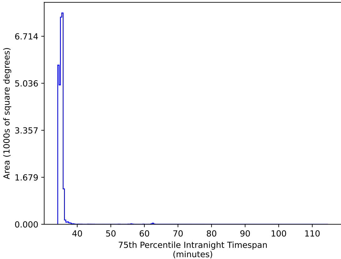
baseline_v3.3_10yrs All sky all bands: 75th Percentile Intranight Timespan
