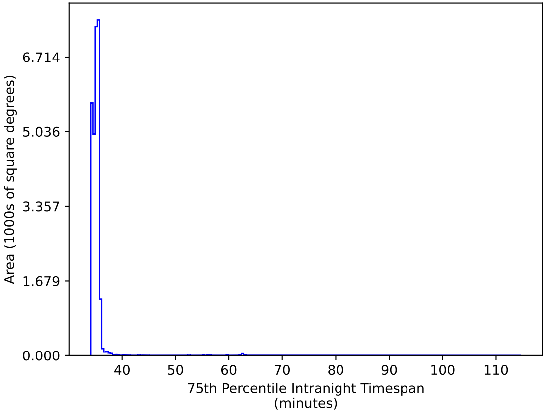
baseline_v3.3_10yrs All sky: 75th Percentile Intranight Timespan
