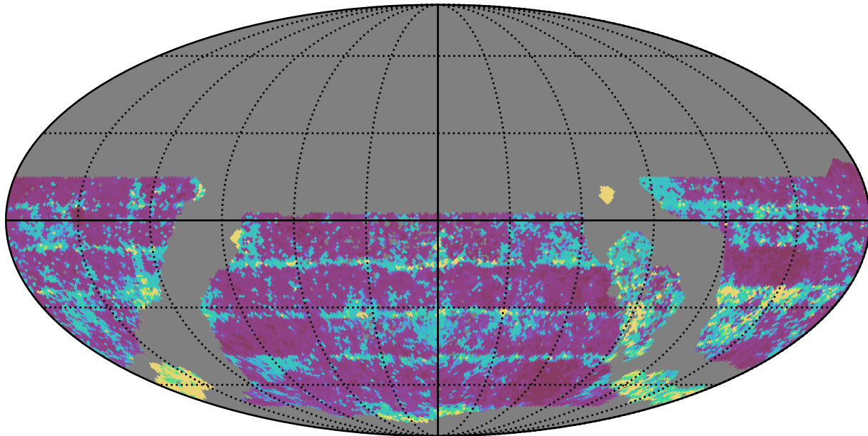
baseline_v3.3_10yrs WFD z band: 20thPercentile Inter-Night Gap
