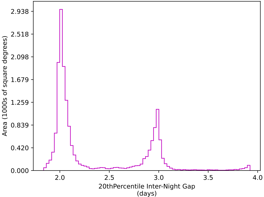
baseline_v3.3_10yrs WFD z band: 20thPercentile Inter-Night Gap
