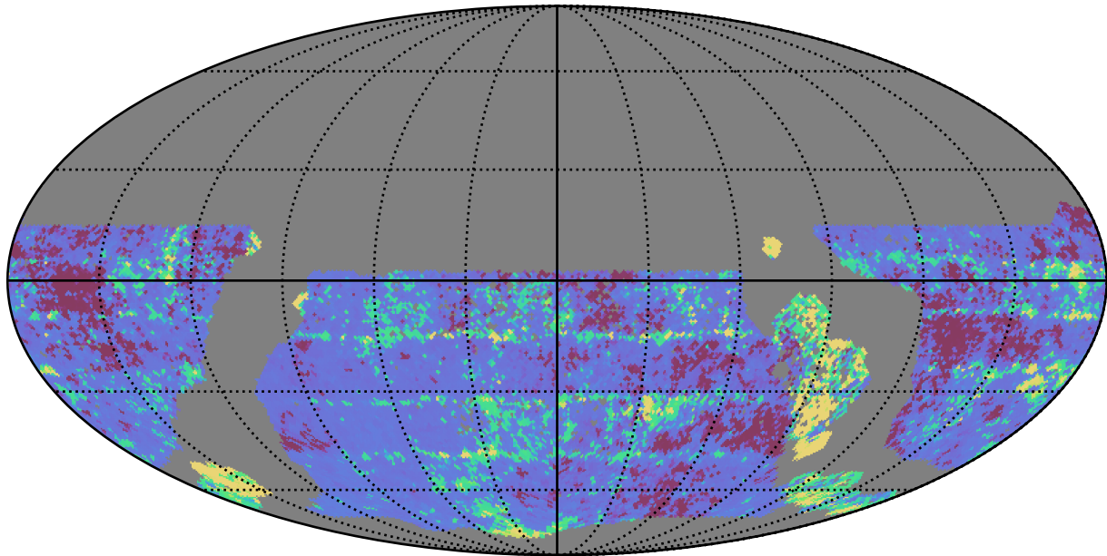
baseline_v3.3_10yrs WFD y band: 20thPercentile Inter-Night Gap
