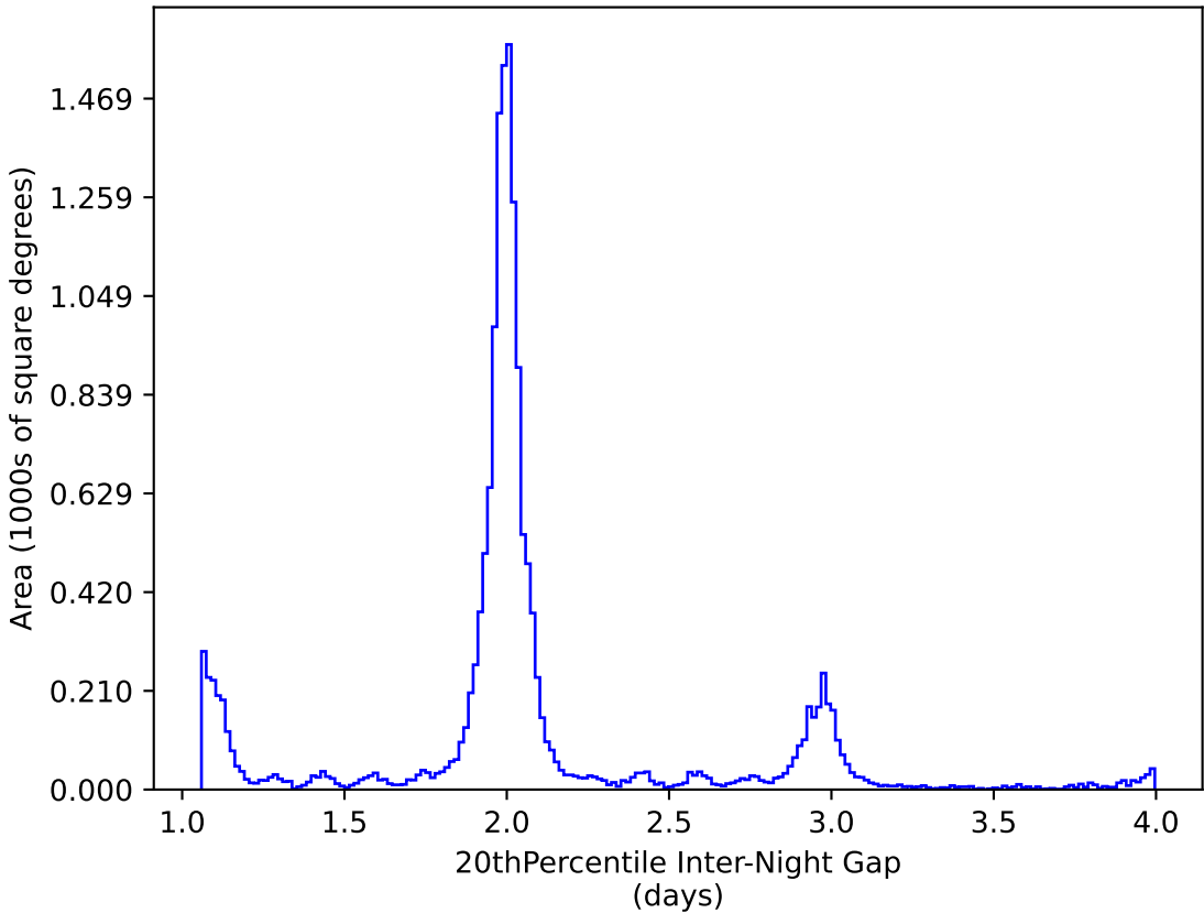
baseline_v3.3_10yrs WFD y band: 20thPercentile Inter-Night Gap
