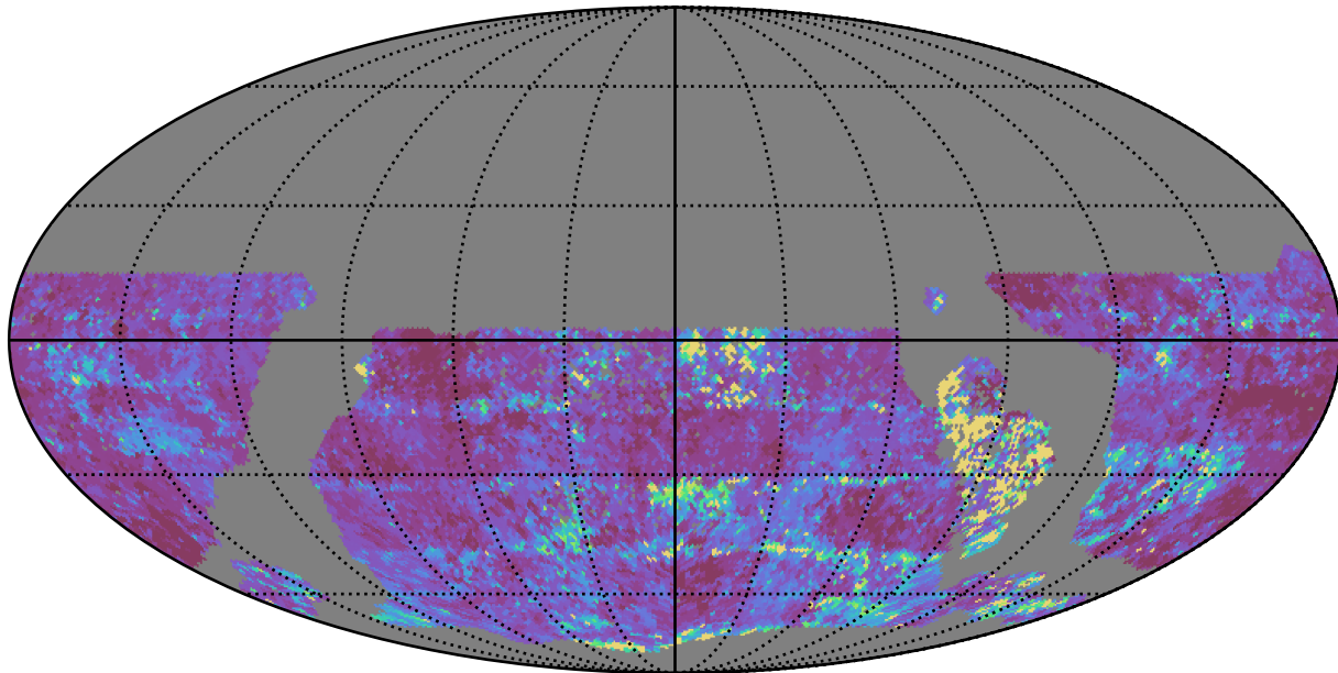
baseline_v3.3_10yrs WFD u band: 20thPercentile Inter-Night Gap
