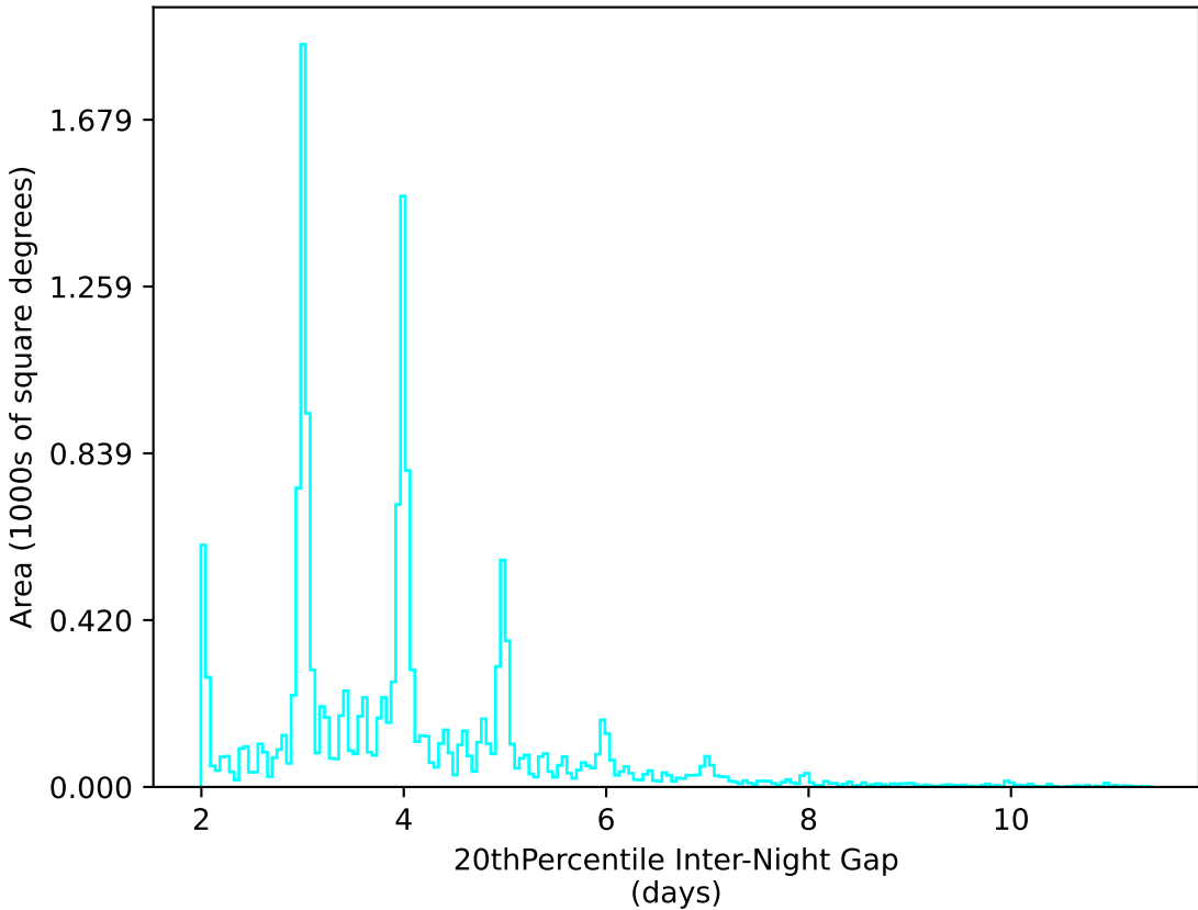
baseline_v3.3_10yrs WFD u band: 20thPercentile Inter-Night Gap
