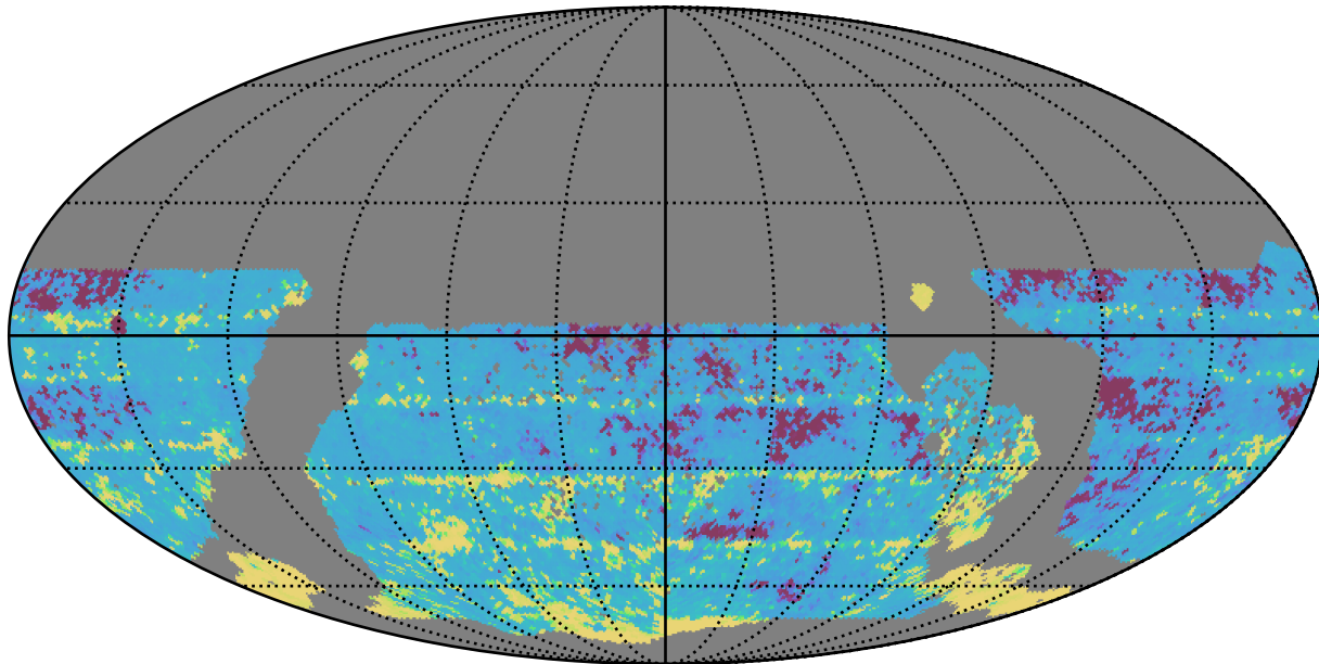
baseline_v3.3_10yrs WFD r band: 20thPercentile Inter-Night Gap
