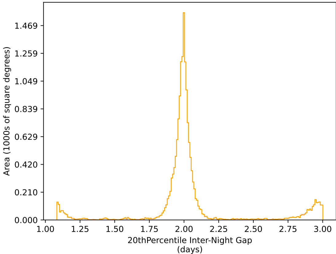
baseline_v3.3_10yrs WFD r band: 20thPercentile Inter-Night Gap
