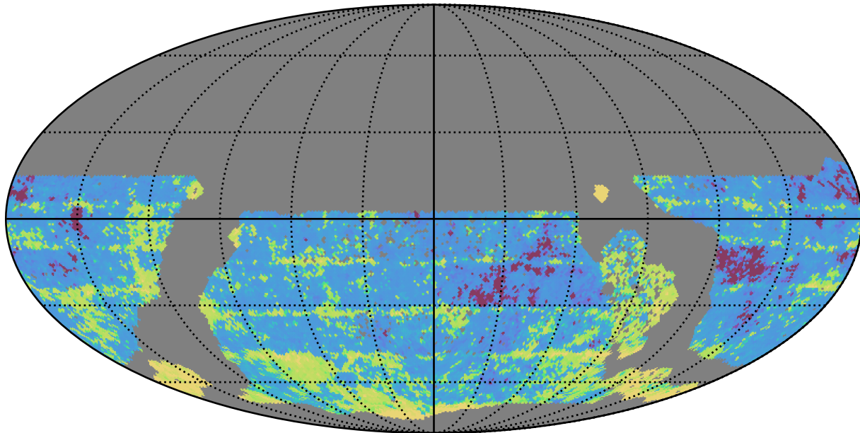
baseline_v3.3_10yrs WFD i band: 20thPercentile Inter-Night Gap
