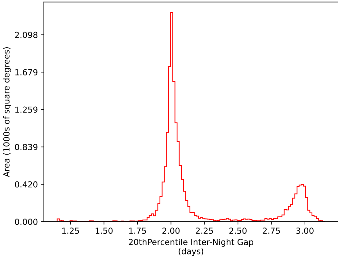
baseline_v3.3_10yrs WFD i band: 20thPercentile Inter-Night Gap
