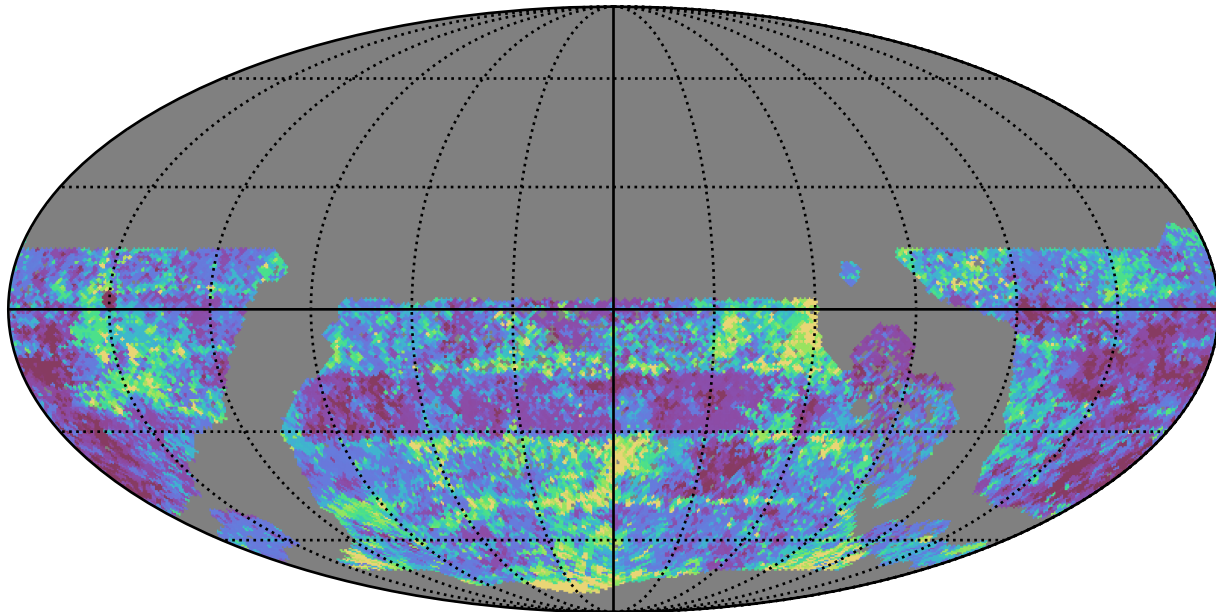
baseline_v3.3_10yrs WFD g band: 20thPercentile Inter-Night Gap
