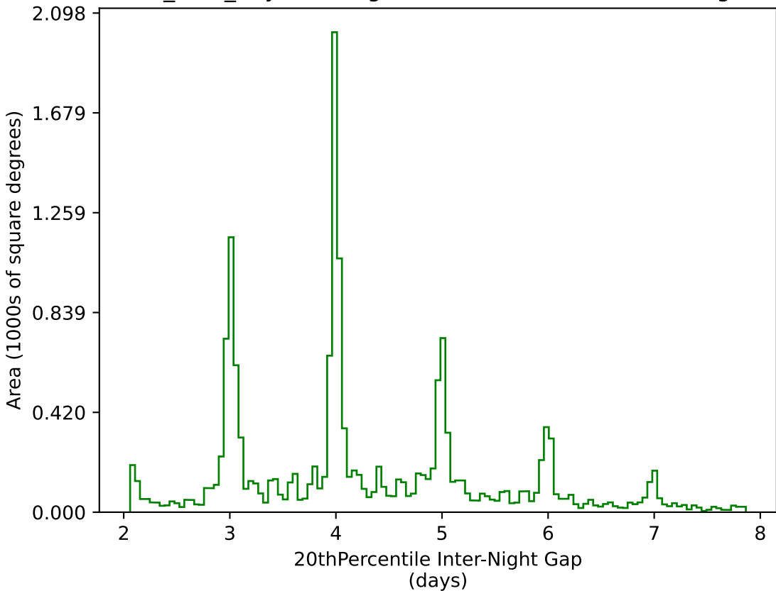
baseline_v3.3_10yrs WFD g band: 20thPercentile Inter-Night Gap
