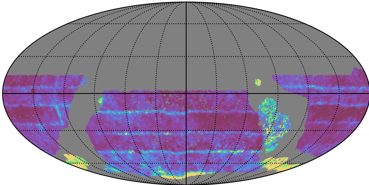
baseline_v3.3_10yrs WFD all bands: 20thPercentile Inter-Night Gap
