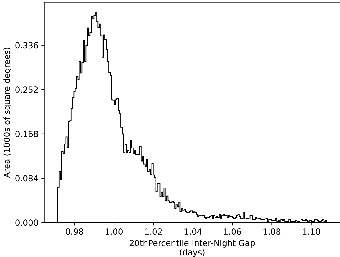
baseline_v3.3_10yrs WFD all bands: 20thPercentile Inter-Night Gap
