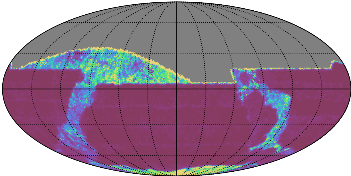
baseline_v3.3_10yrs All sky z band: 20thPercentile Inter-Night Gap
