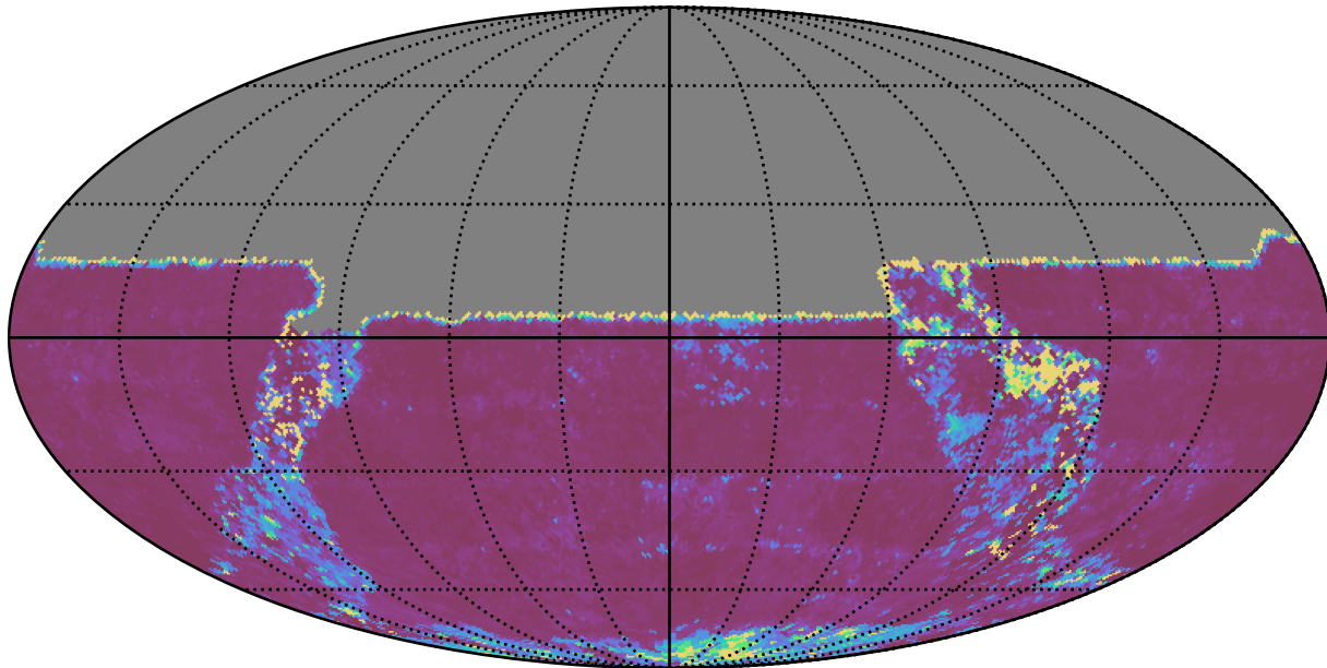
baseline_v3.3_10yrs All sky u band: 20thPercentile Inter-Night Gap
