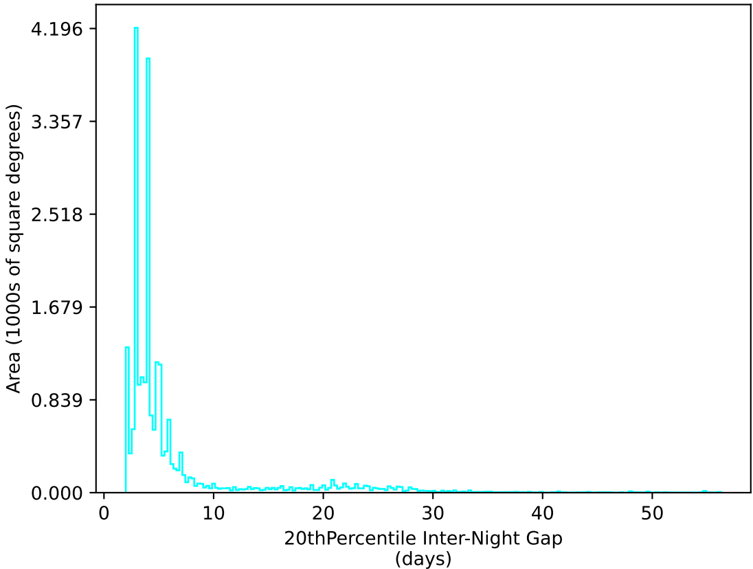
baseline_v3.3_10yrs All sky u band: 20thPercentile Inter-Night Gap
