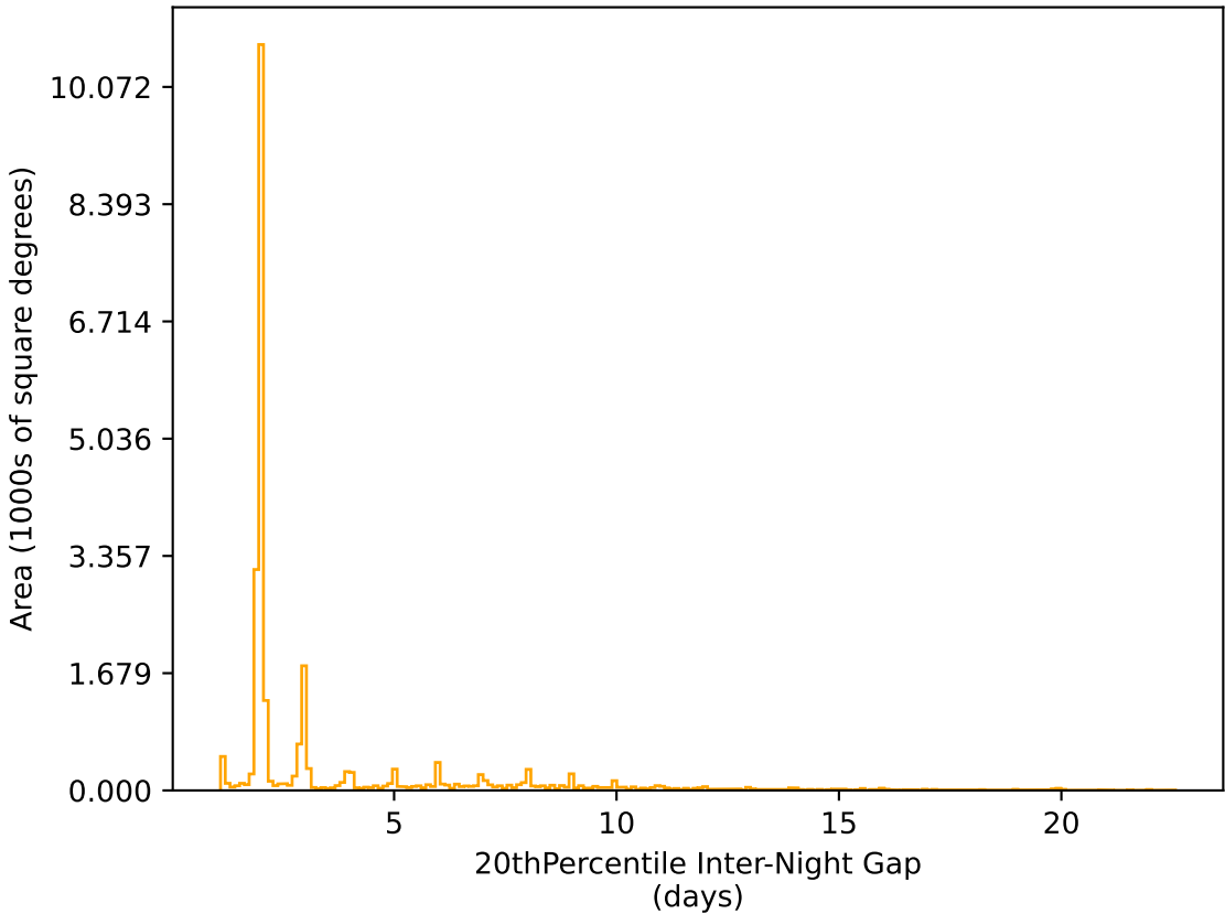
baseline_v3.3_10yrs All sky r band: 20thPercentile Inter-Night Gap
