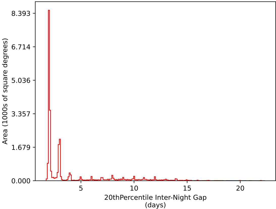
baseline_v3.3_10yrs All sky i band: 20thPercentile Inter-Night Gap
