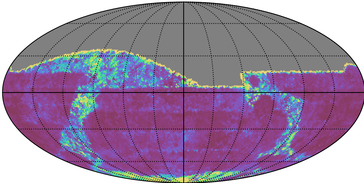
baseline_v3.3_10yrs All sky g band: 20thPercentile Inter-Night Gap
