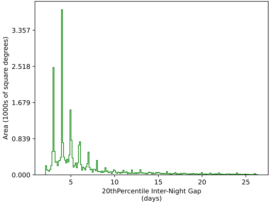
baseline_v3.3_10yrs All sky g band: 20thPercentile Inter-Night Gap
