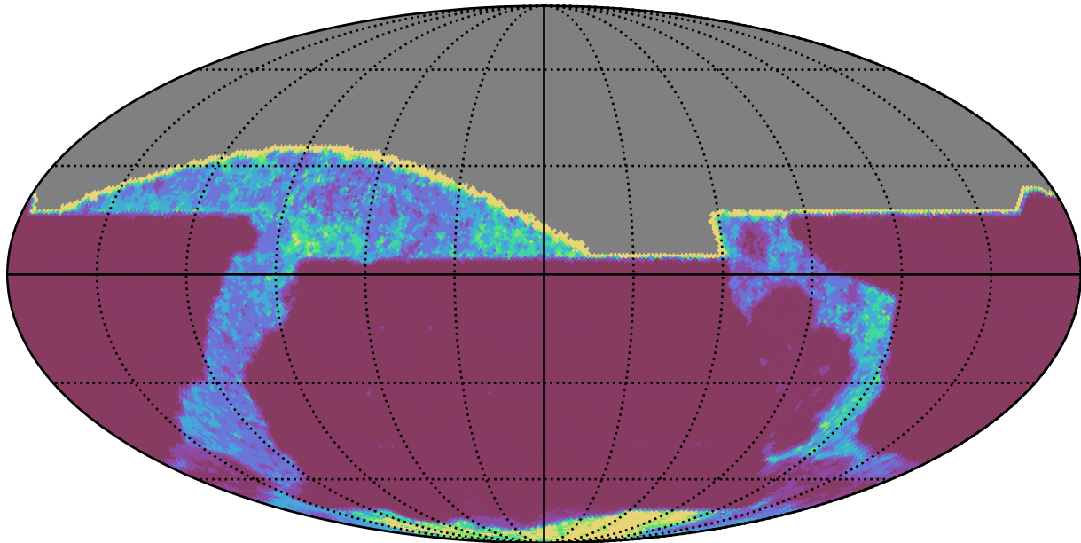
baseline_v3.3_10yrs All sky all bands: 20thPercentile Inter-Night Gap
