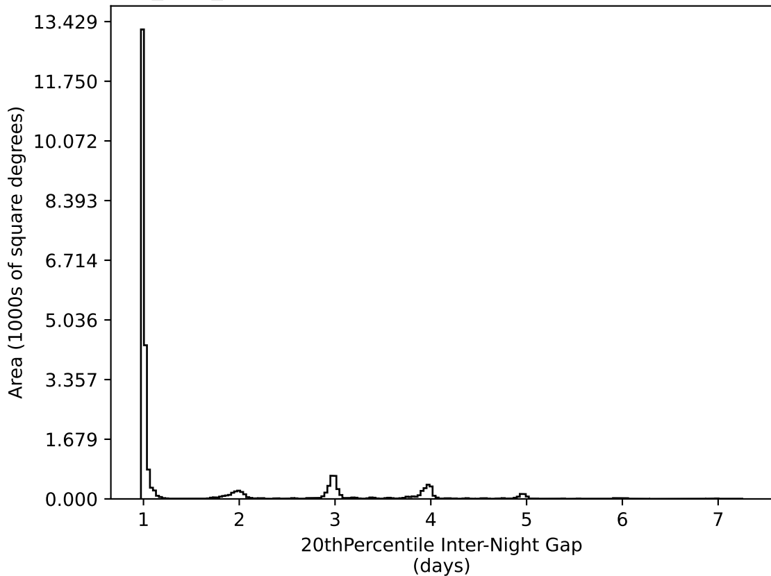
baseline_v3.3_10yrs All sky all bands: 20thPercentile Inter-Night Gap
