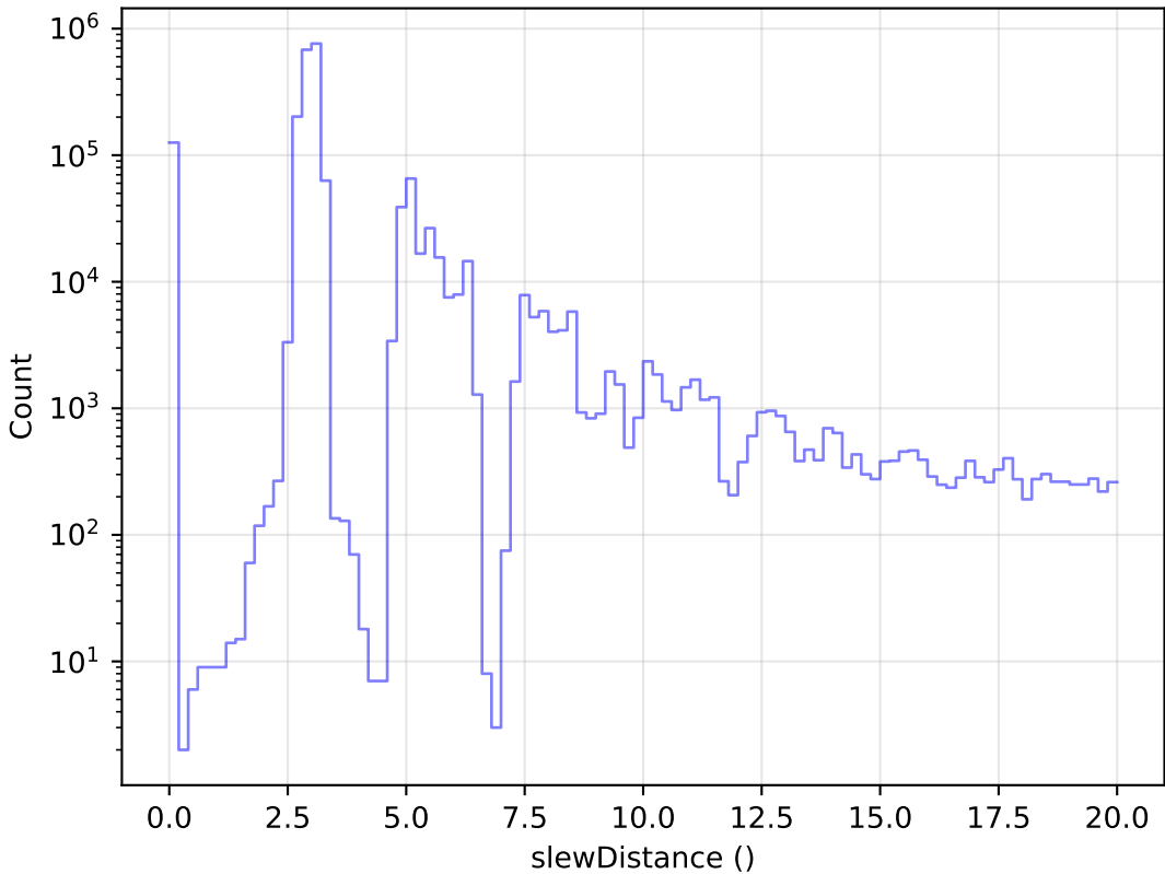
baseline_v3.3_10yrs All visits: Zoom Slew Distance Histogram
