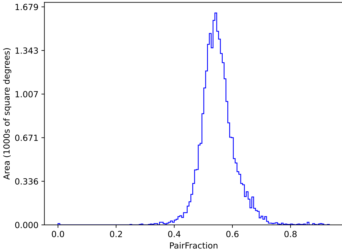
baseline_v3.3_10yrs (g or r or i): PairFraction
