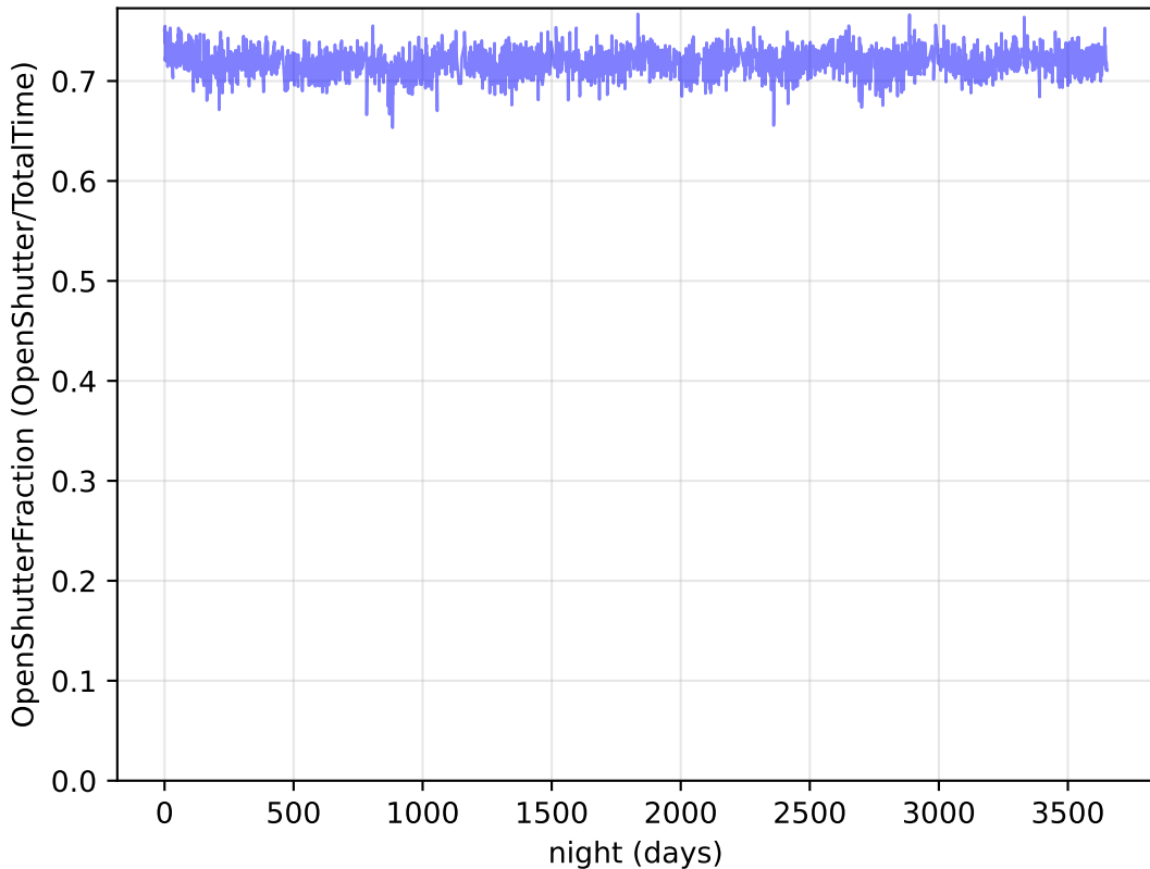
baseline_v3.3_10yrs : OpenShutterFraction
