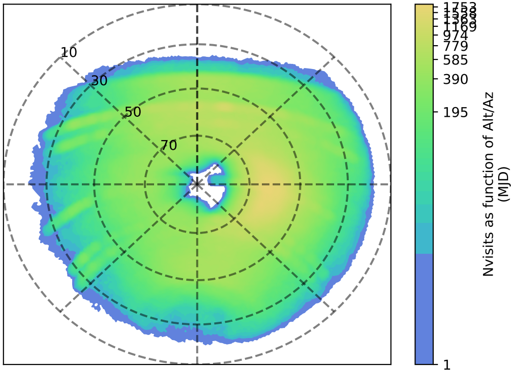
baseline_v3.3_10yrs y: Nvisits as function of Alt/Az
