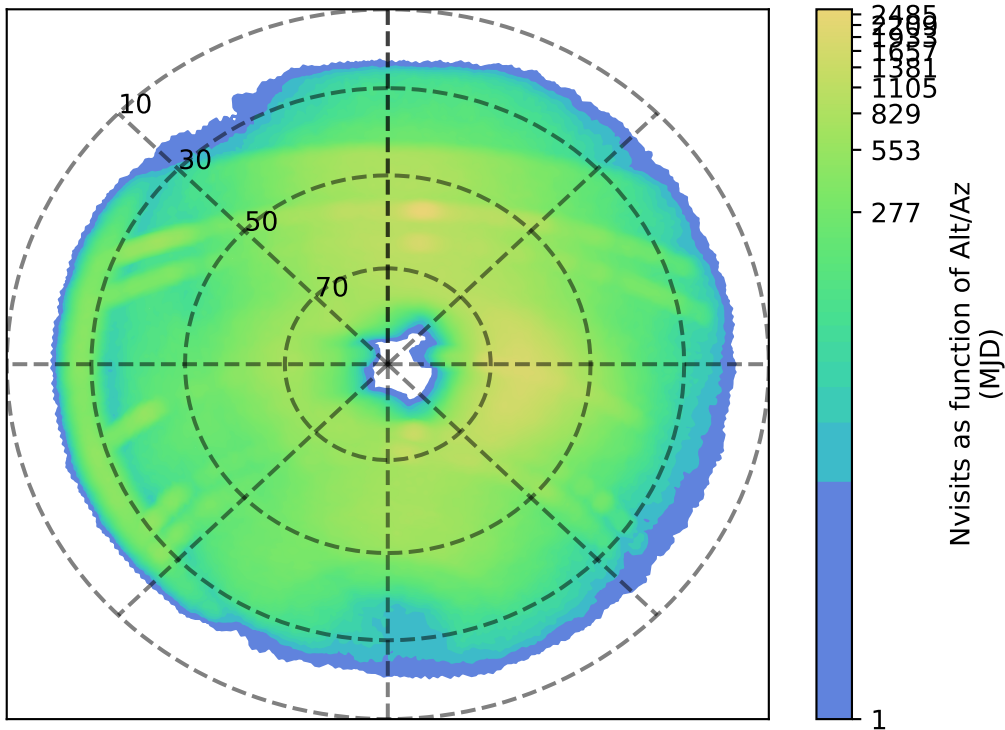
baseline_v3.3_10yrs r: Nvisits as function of Alt/Az
