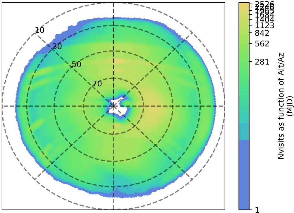
baseline_v3.3_10yrs i: Nvisits as function of Alt/Az
