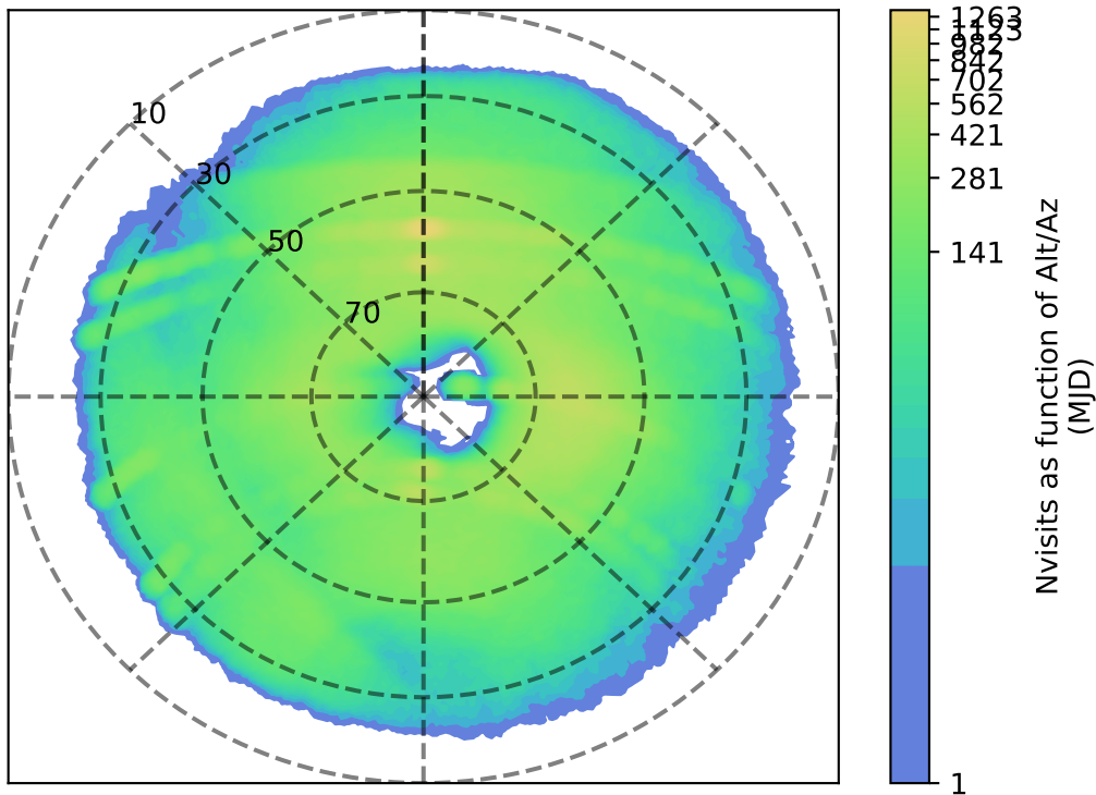
baseline_v3.3_10yrs g: Nvisits as function of Alt/Az
